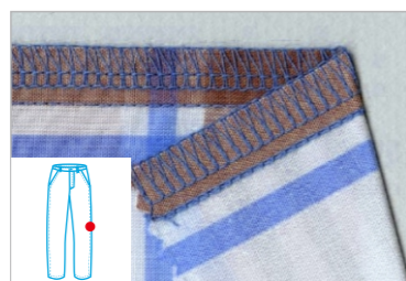
Six Threads Basic Stitch C6-6-03/333/AT
