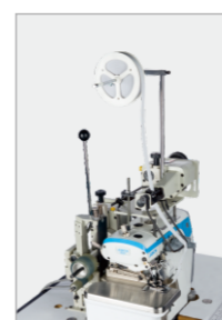
Rear Puller + Elastic Attaching Device
