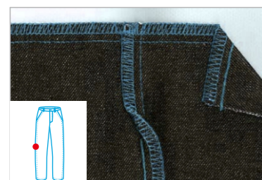
Five Threads Heavy Duty Stitch C6-5-M04/435/AT
