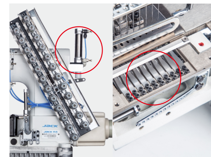
Auto presser foot lifter, more laborsaving, auto trimming, higher efficiency
