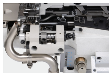
Bottom Hemming (Left-side Cutter)
