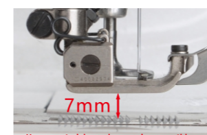
Heavy materials can be sewn smoothly Height of presser foot form 5mm up to 7mm
