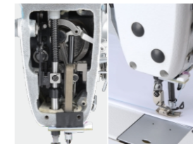
Feed smoothly; Avoid of layers offset.
