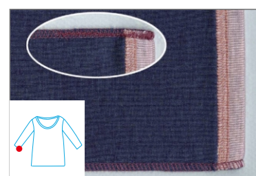
Three Threads Pneumatic Back Latch Seaming C6-3-82/233/BK
