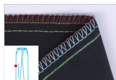
Five Threads Basic Stitch(5x5) C6-03/233/KH
