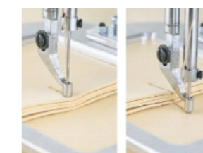
Intelligent central presser foot
